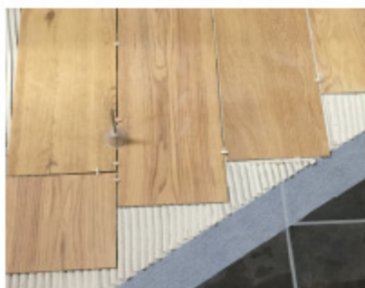
Step 4: Laying tile with spacers
